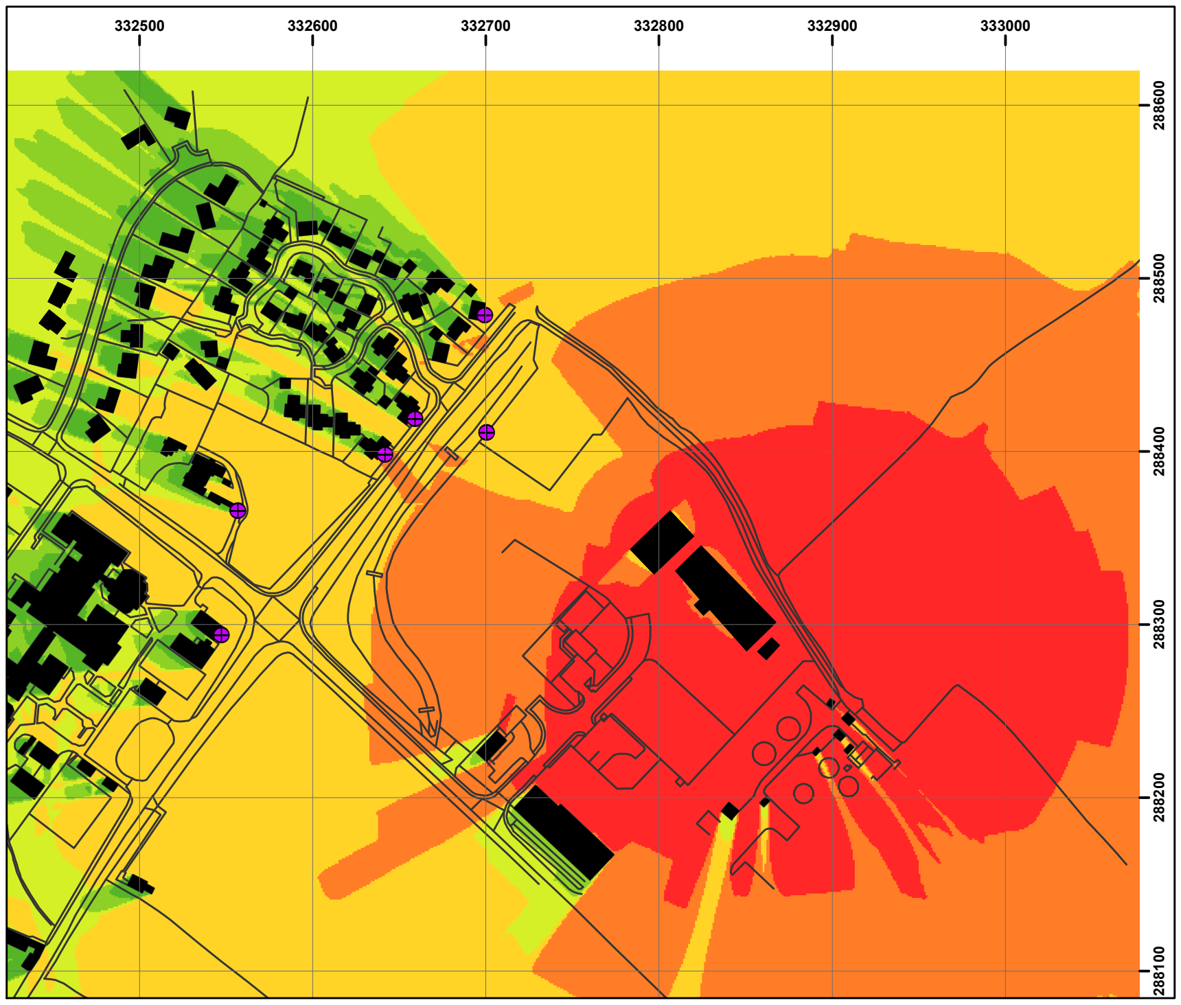
Figure A1 Noise Contour Plot
